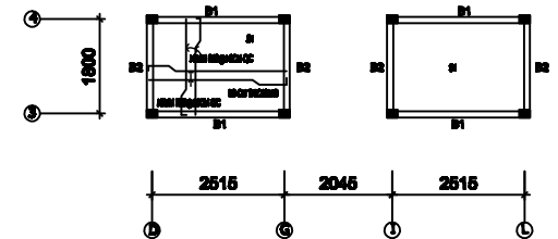
LAYOUT OF STAIRCASE HEAD ROOM ROOF SLAB DETAILS @ 9.00M
