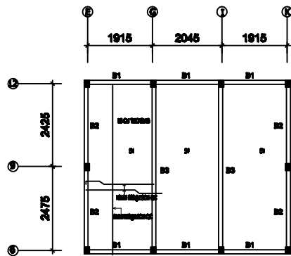
LAYOUT OF TRAINING ROOM ROOF SLAB DETAILS @ 7.80M
